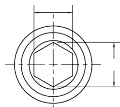
Hexagonal 01.(内六角孔)
