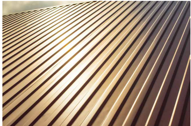
Figure 3: Installation of Exposed Fastener Metal Roof System
